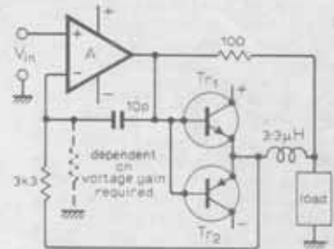
Fig. 2. Basic diagram of principal elements.
