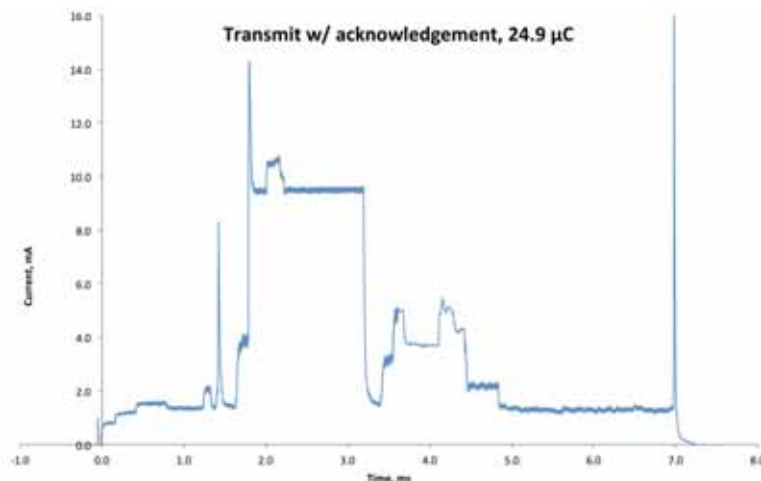
Figure 1: Energy to transmit a short 802.15.4 packet and receive an acknowledgement
