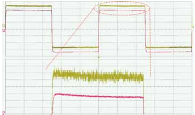
Figure 2: Multiple-acquisition averaging is an attempt at improving vertical precision in software. In this example, a continuous square-wave signal is averaged from the green trace into the cleaner magenta trace seen in the zoom view
