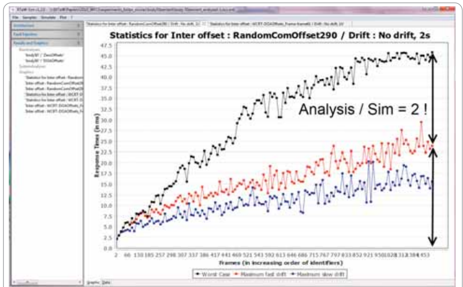
Figure 2: Worst-case response times (by decreasing priority of the frames) obtained by analysis (black curve) versus maximum values collected during long simulation runs for two ECU clock drift values (screenshot of RTaW-Sim [2])
