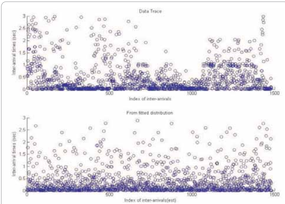
Figure 4: On the two graphs, the X-axis shows the index of the aperiodic frames while the Y-axis is the time between two successive aperiodic transmissions. The upper graph is a real data trace collected while driving (only the aperiodic frames). The lower graph is an artificial data trace generated with a probabilistic model of the aperiodic frames (here Weibull interarrivals with parameters fitted with maximum-likelihood estimation using the real data trace). The probabilistic model can be used both for simulation and worst-case analysis, as done in [14]
