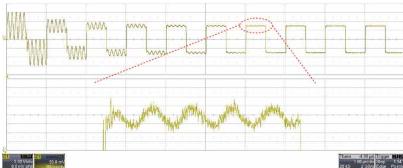
Figure 4: Because HD4096 technology achieves true 12-bit resolution through hardware improvements and not through averaging or filtering, the user no longer needs to average samples by combining multiple acquisitions into a single trace. Compare this HDO screen image with Figure 2, which illustrates the result of multiple-acquisition averaging
