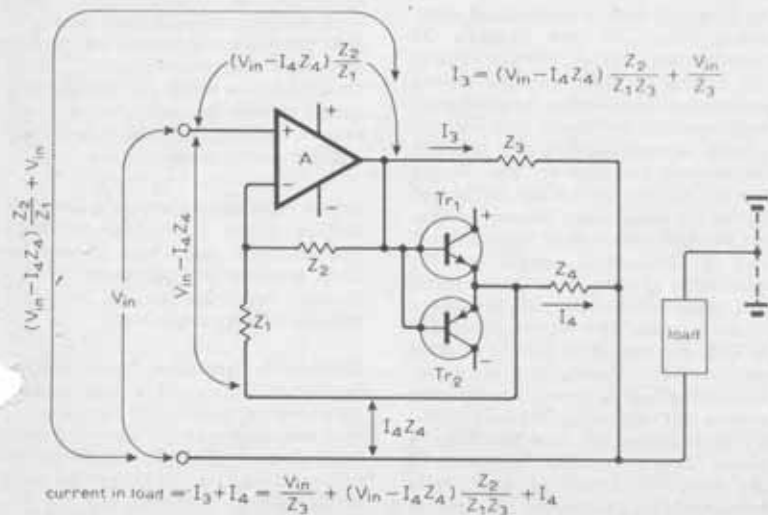
Fig. 1. Basic circuit parameters.
