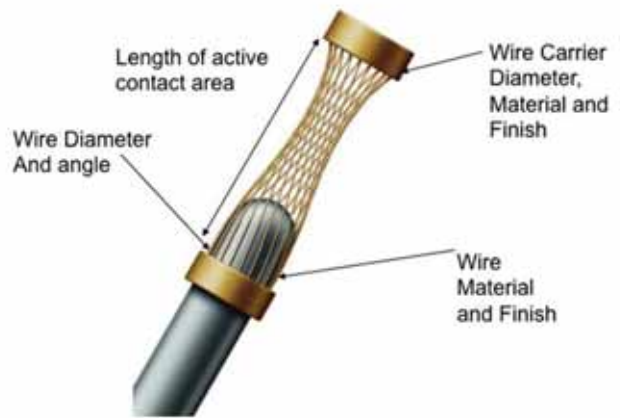
Figure 2: Design parameters of the Hyperboloid socket contact
