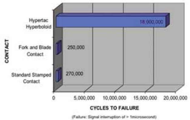
Figure 3: Fretting corrosion characteristic of Hyperboloid contacts
