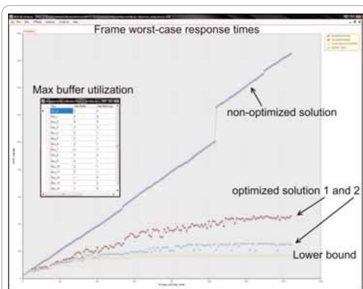
Figure 1: Screenshot of NETCAR-Analyzer, showing maximum buffer utilization and CAN frame worst-case response times (by decreasing priority) for different offset configurations. This graph shows the typical gain one can expect with offsets
