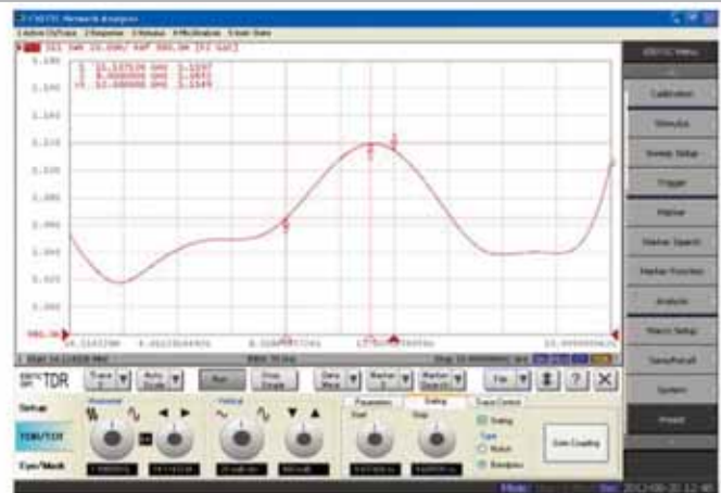
Figure 4: VSWR for a mated pair with Hypertac coaxial sockets for both inner and outer contacts
