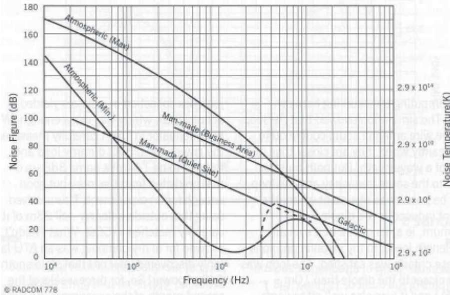
Fig. 11. Graph plotting noise levels and frequencies, showing atmospheric noise least at relevant frequencies. (Source: RadCom, RSGB, after MacKeand).
