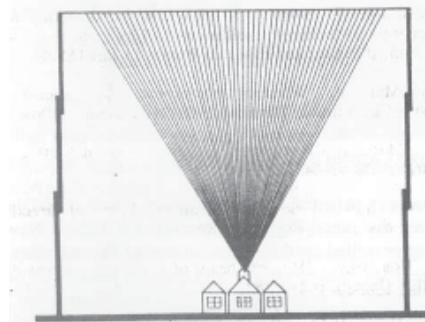
Fig. 17. A schematic drawing of the jury-rigged antenna at Poldhu, which was a vertical fan of about 54 wires [30] erected after a storm took down a larger, planned cone-like multi-wire antenna.
