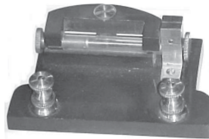
Fig. 7. The actual Mercury Detector used by Marconi at St. John's, now on display at the Science Museum, London (photo Bart Lee). Lane Upton functionally replicated Marconi's detector based in part on this photo.
